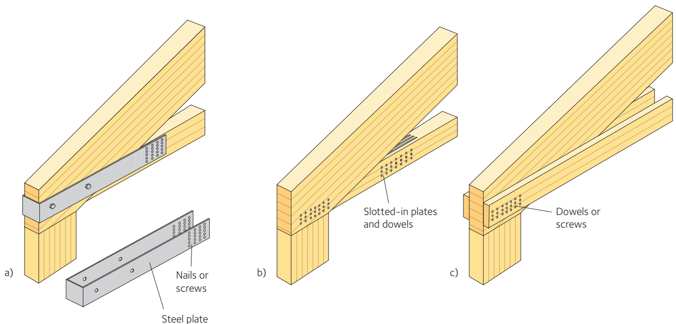
Figure 9.7 Anchoring of glulam tension tie to the rafter
