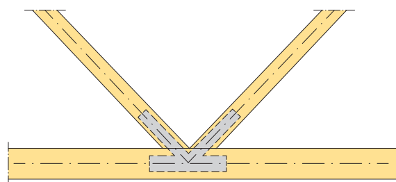
Figure 14.38 Truss joint based on slotted-in steel plates
