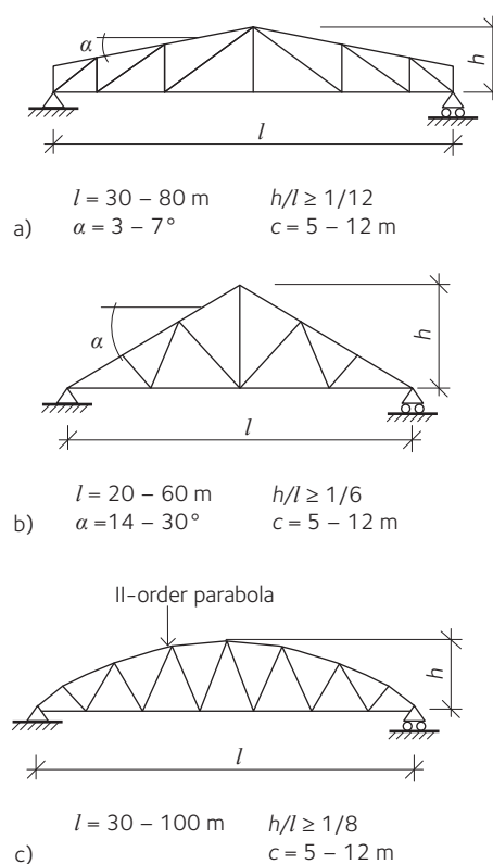
Figure 8.7 Preliminary design of three different truss types. “c” is the centre-to-centre distance between adjacent trusses.
