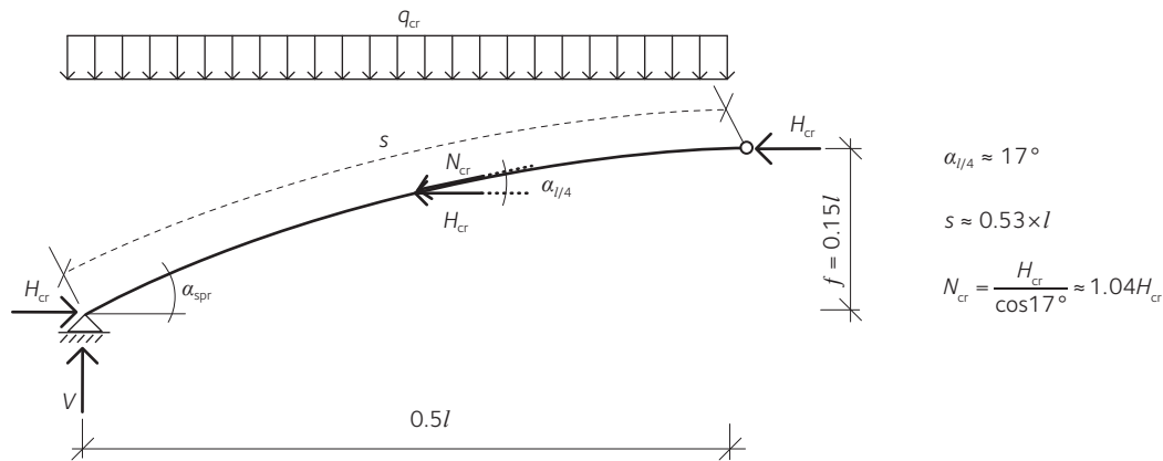
Figure 11.14 Forces acting on one half of a three-hinged arch. \alpha_{l/4} is the angle between the axis of the arch and a horizontal line at the quarter point. s is the length of the semi-arch. N_{cr} is the Euler buckling load calculated at the quarter point of the arch.
