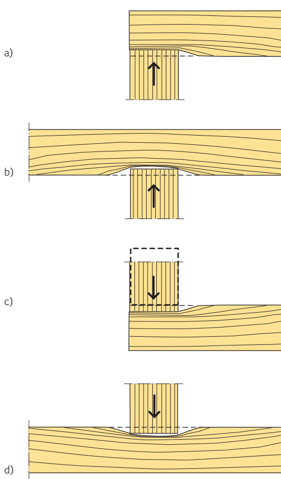
Figure 4.7 Bearing failure perpendicular to the grain
