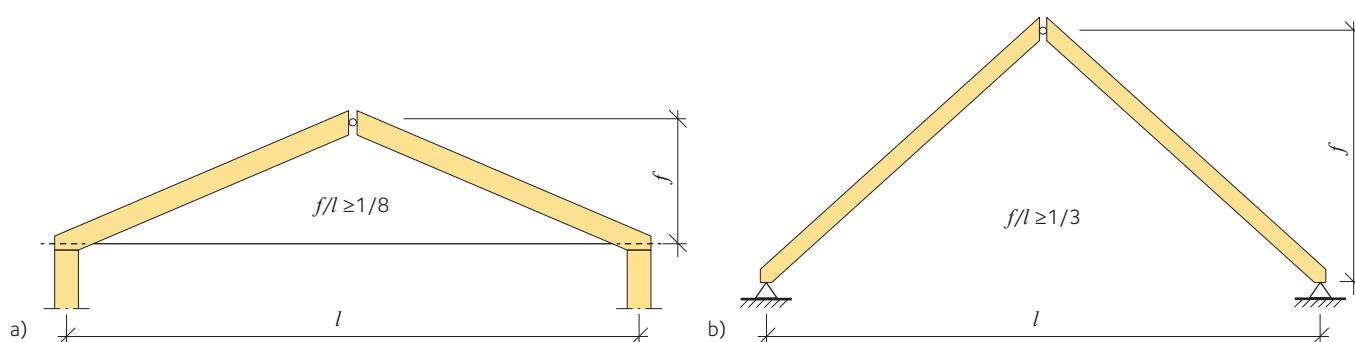
Figure 9.1 Three-hinged trusses
