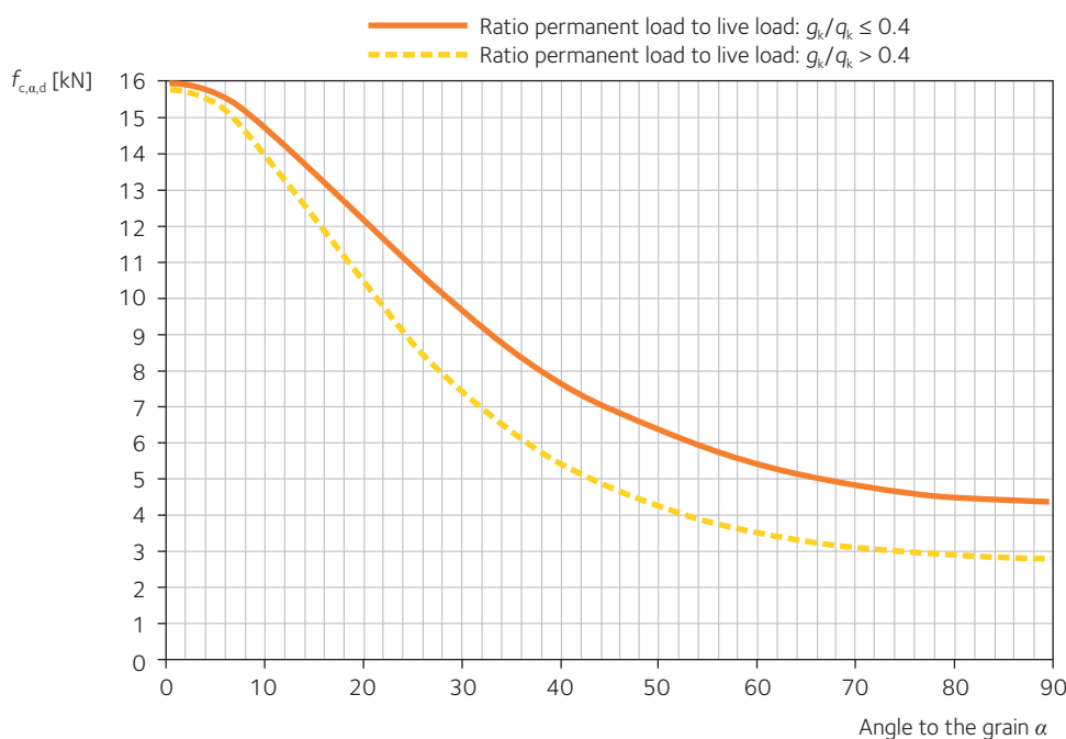
Figure 4.12 Strength for glulam member loaded in compression at an angle \alpha to the grain
