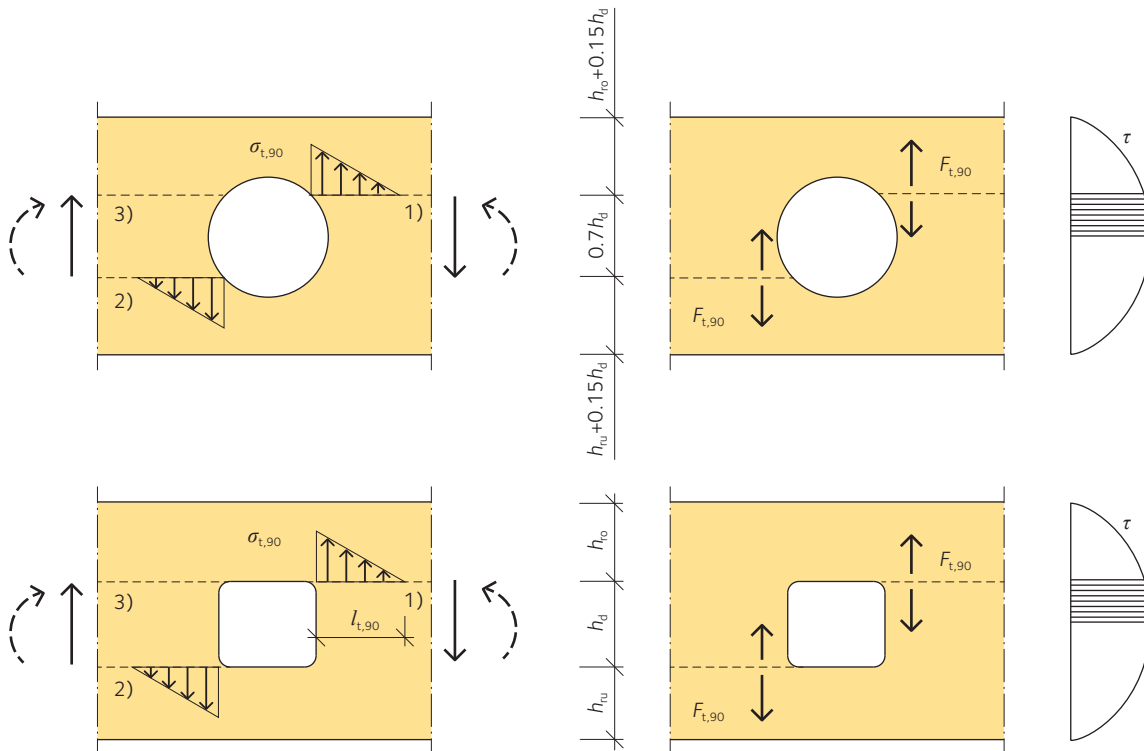
Figure 5.6 Location of critical planes concerning cracking for rectangular and circular holes
