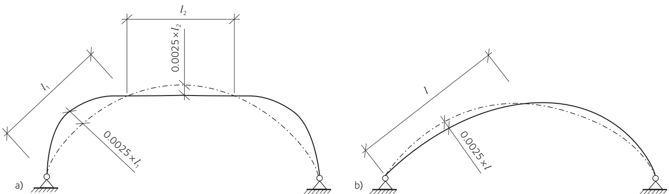
Figure 11.15 Recommended assumptions for initial deviation in the geometry of arches according to EC5
