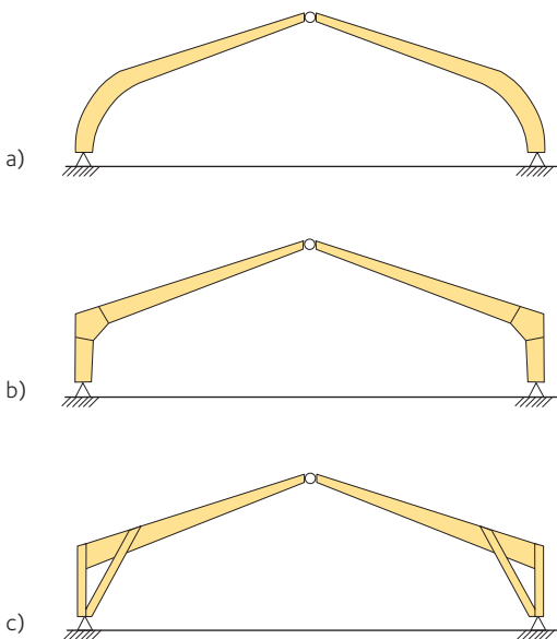
Figure 10.1 Examples of three-hinged portal frames
