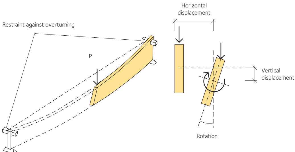
Figure 4.2 Lateral-torsional buckling of a simply supported beam
