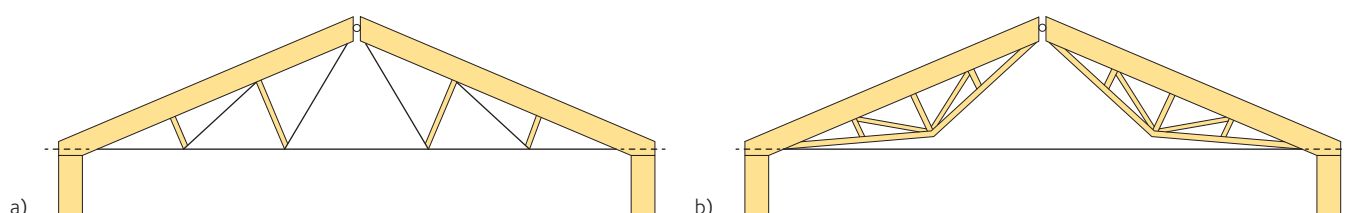
Figure 9.2 Three-hinged trusses with reinforced ties
