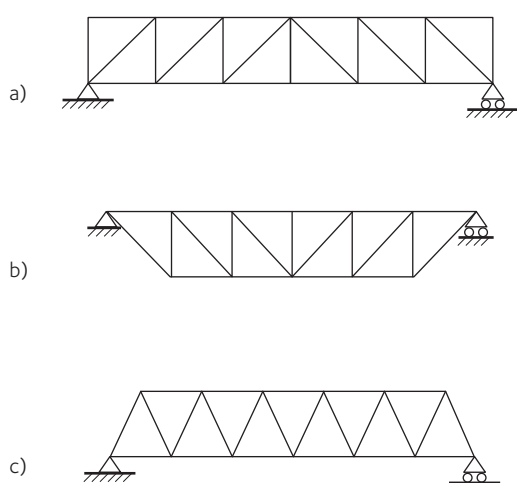
Figure 8.3 Examples of parallel-chord trusses
