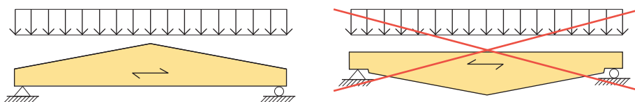
Figure 7.4 Left: compression perpendicular to the grain occurs at the tapered edge.
