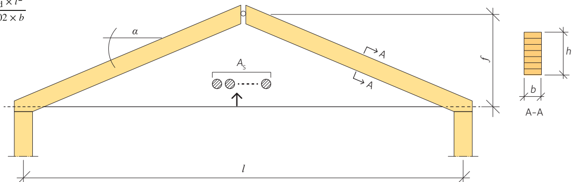
Figure 9.5 Typical three-hinged frame with steel tension tie
