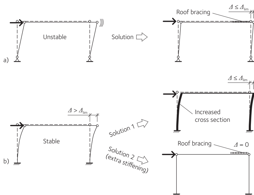
Figure 13.10 Effect of longitudinal roof bracing on the lateral displacement of post-and-beam structures
