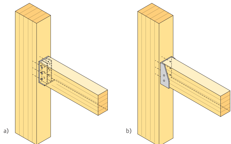
Figure 14.20 Two different types of beam hangers
