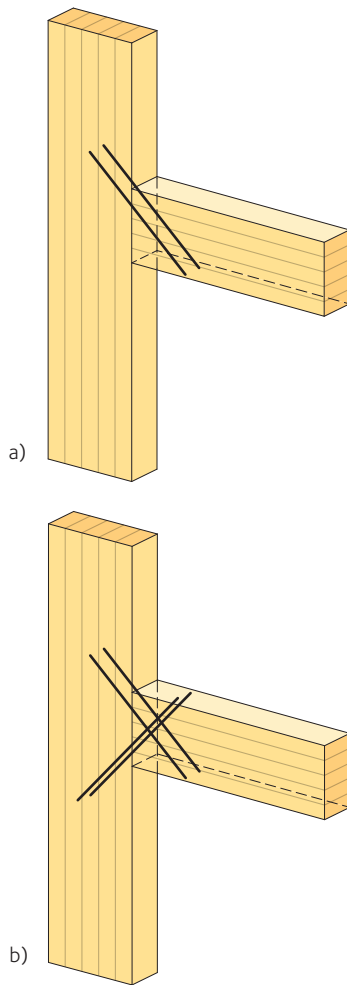
Figure 14.19 Beam-to-column connection with self-tapping screws
