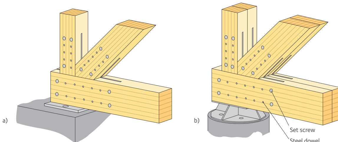
Figure 8.21 Two examples of nodes at the support of trusses using steel plates and dowels
