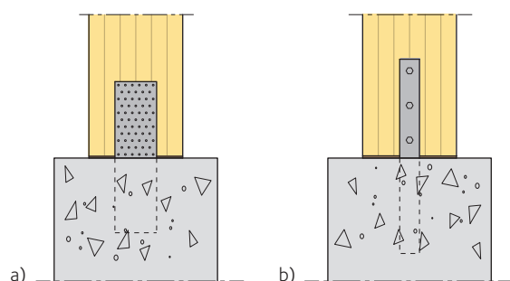
Figure 16.22 Pinned column base
