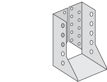
Figure 16.28 Hanger with internal flanges
