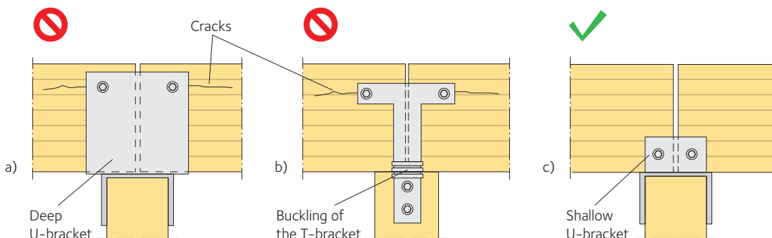
Figure 15.2 Beam-to-column connections
