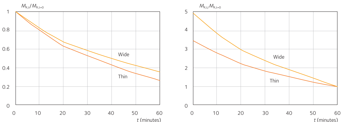
Figure 16.19 Decrease of resistant bending moment for “wide” and “thin” glulam sections
