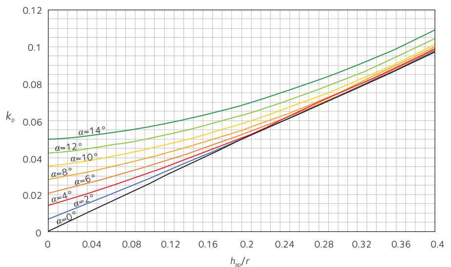
Figure 7.12 Factor k_p according to Eurocode 5 for different values of h_{ap}/r , glulam class GL30c
