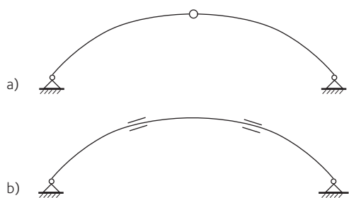
Figure 11.3 Suitable placing of joints in arch structures
