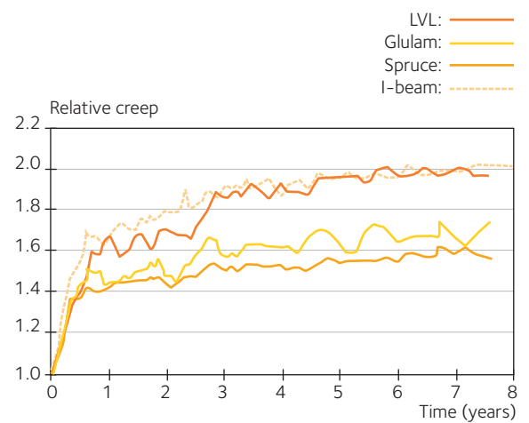
Figure 6.3 Relative creep in sheltered environment (relative creep = beam deflection at time t / initial deflection). Stress level 2 MPa. After Alpo Ranta-Maunus & Markku Korttesmaa (2000).
