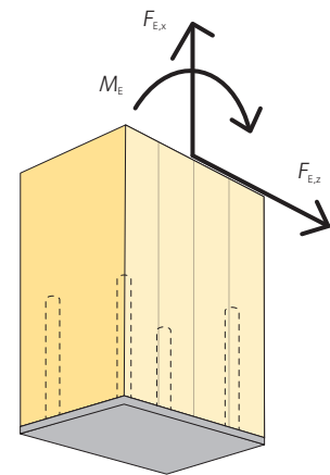
Figure 14.18 Fixed column base with bonded-in rods
