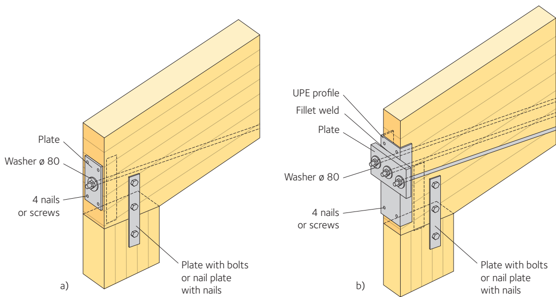
Figure 9.6 Anchoring of steel tension tie to the rafter
