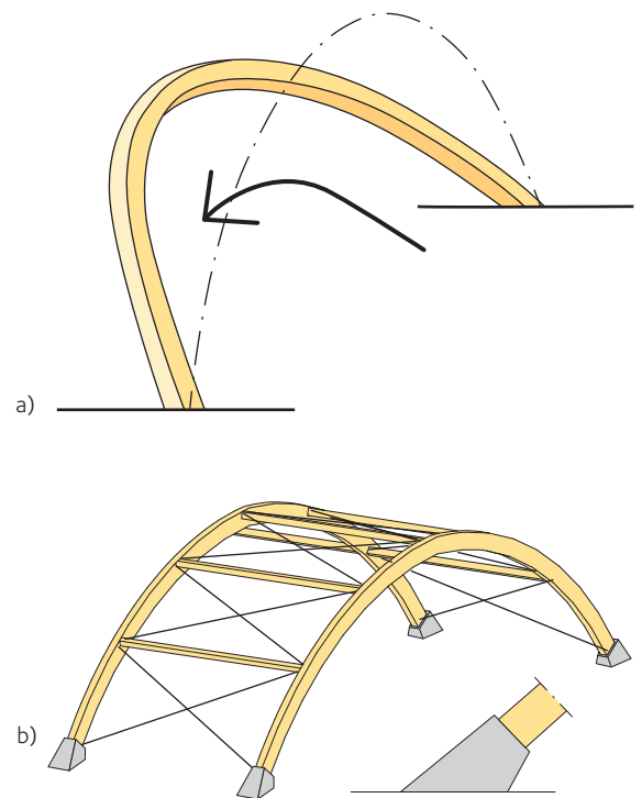
Figure 11.10 Considerations concerning the lateral behaviour of arches during erection
