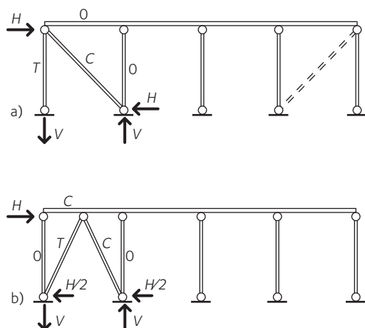
Figure 13.17 Bracing by timber members
