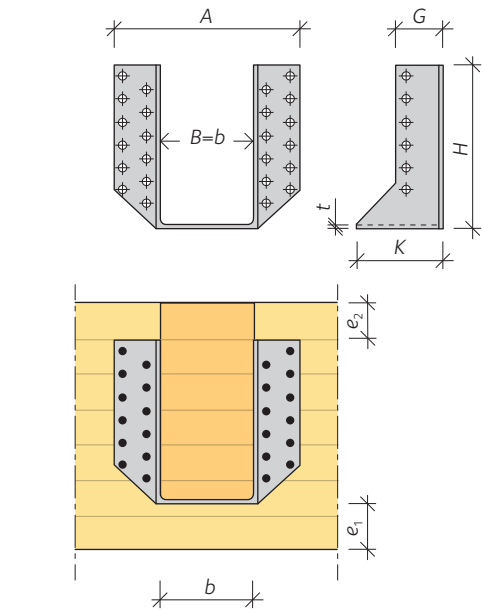
Figure 16.27 Connection of secondary beam with standard beam hanger: R30
