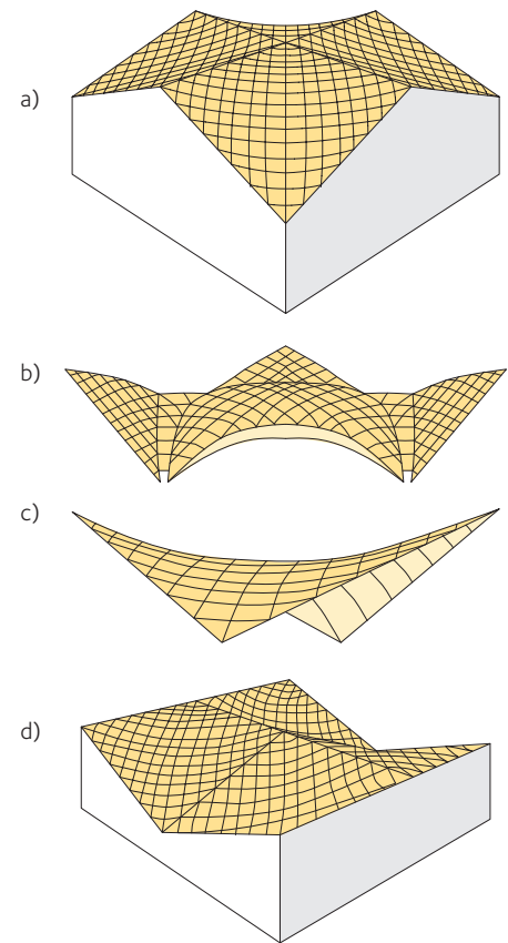
Figure 3.18 Shells
