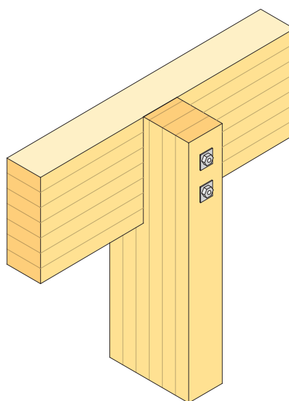
Figure 14.30 Column top with a recessed beam and through bolts
