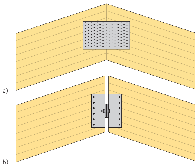
Figure 16.32 Ridge joints
