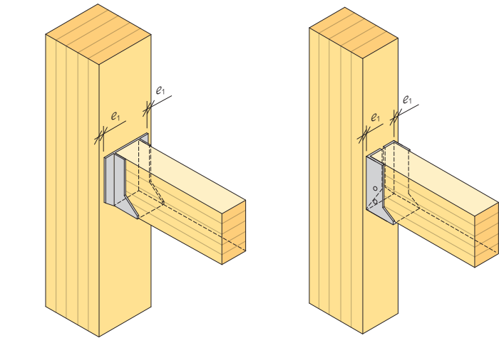
Figure 16.29 Edge spacing for beam-column connection with standard beam hanger: R30 under certain conditions, see table 16.7
