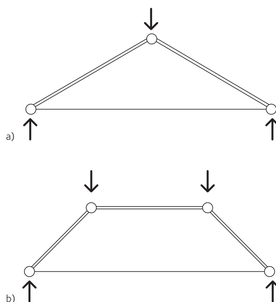
Figure 8.1 Examples of idealised truss arrangements for two different loadings
