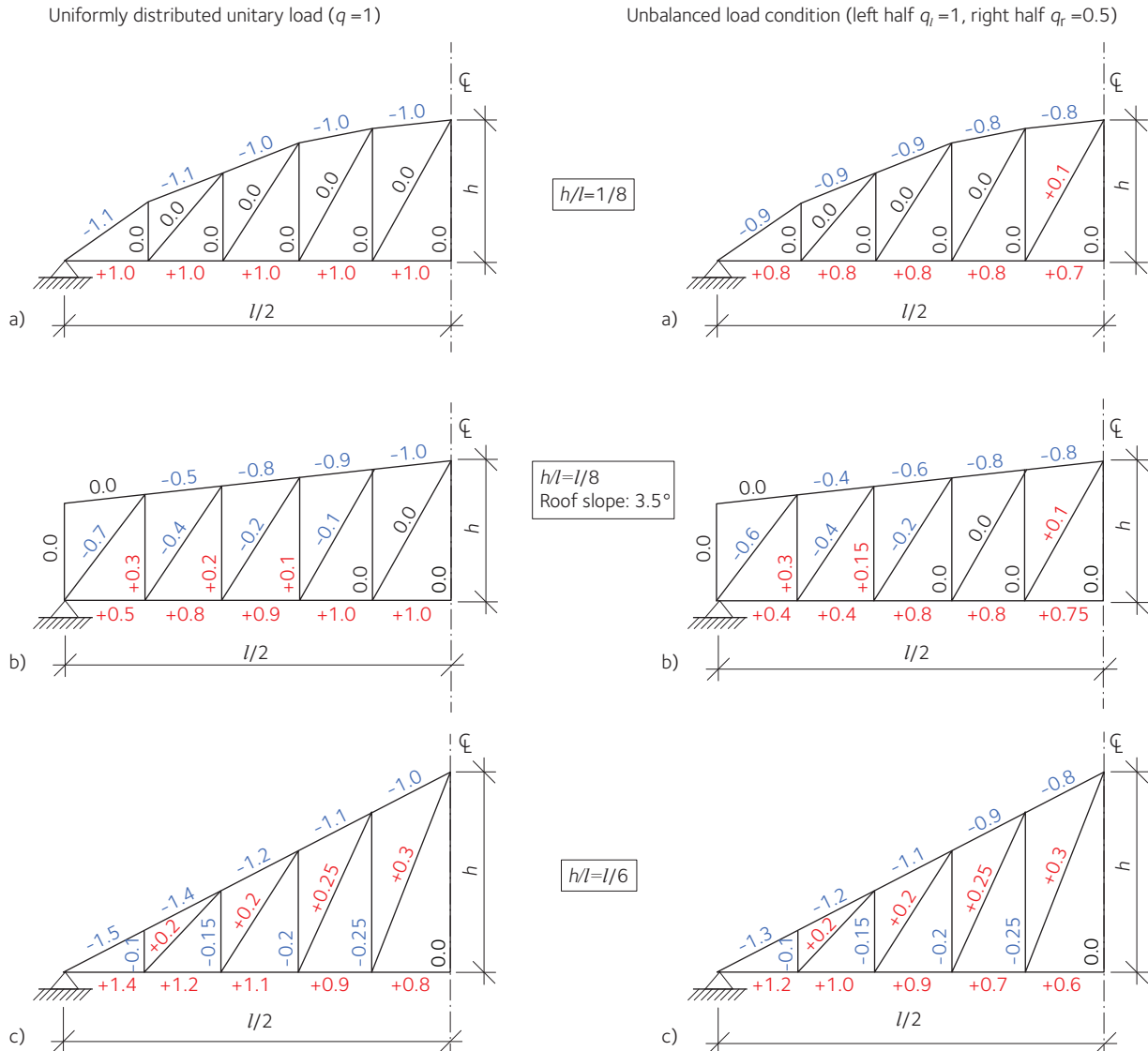
Figure 8.6 Magnitude of normal forces in three different truss types: a) Bowstring, b) pitched trapezoidal and c) pitched triangular (bottom).
