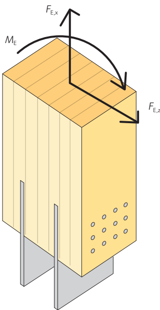
Figure 14.17 Slotted-in steel plates for fixed column base
