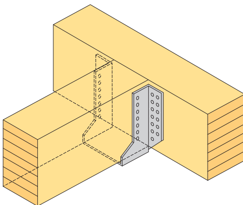
Figure 16.17 a) Connection between joist and main beam, b) protected by means of calcium silicate plates, c) possible alternative to an exposed connection between joist and main beam
