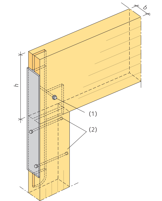
Figure 16.26 Column-beam connection with slotted-in T-profile: R30 or R60 depending on dimensions 1) Through bolt. 2) Through bolt with washer.
