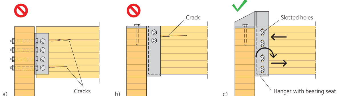
Figure 15.9 Beam-to-beam connections
