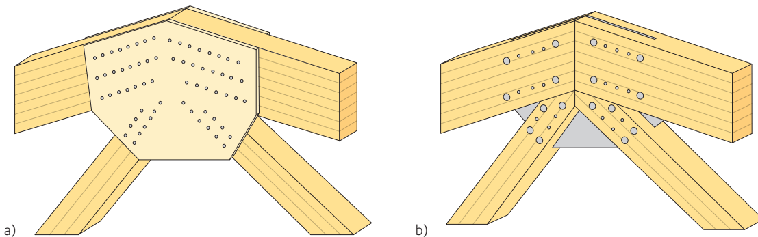
Figure 8.20 Nodes at the ridge of pitched trusses
