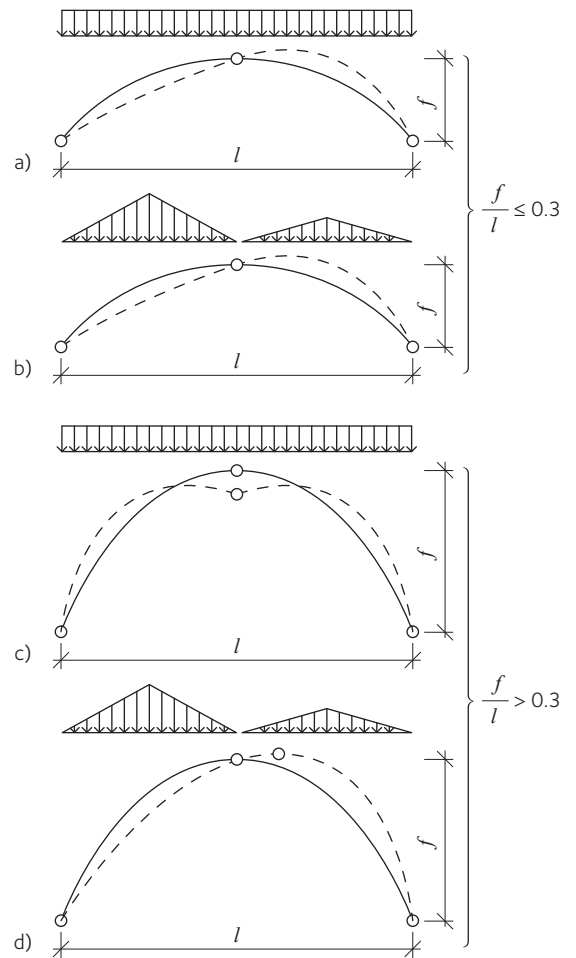
Figure 11.12 In-plane buckling of three-hinged arches
