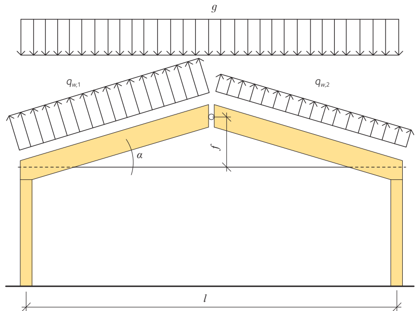
Figure 9.4 Three-hinged truss subjected to self-weight, g , and wind suction, q_{w,1} and q_{w,2}
