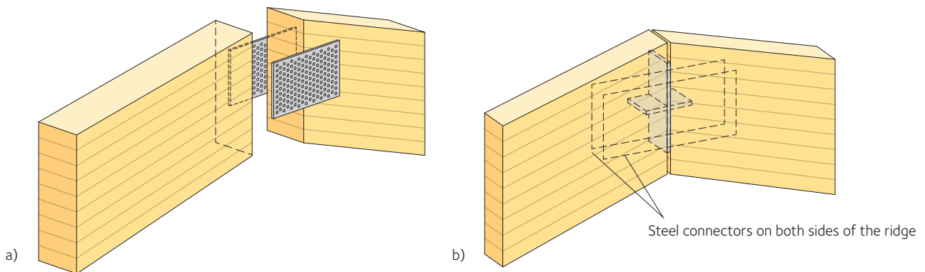
Figure 9.8 Hinged ridge joint a) for moderate shear force at the ridge, b) for large shear force at the ridge.
