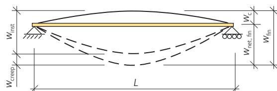
Figure 6.2 Definitions of deflections
