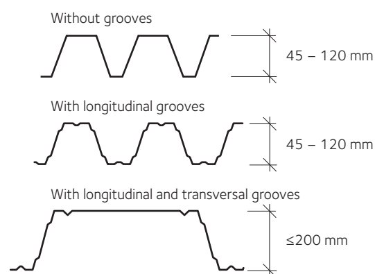
Figure 13.31 Typical cross-section of trapezoidal metal sheeting
