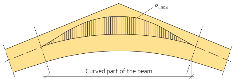
Figure 7.16 Typical distribution of tensile stresses perpendicular to grain in a pitched cambered beam
