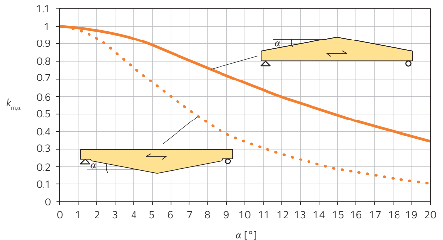
Figure 7.9 Values of k_{m,\alpha} according to Eurocode 5 for different slopes of the tapered edge; Glulam class GL30c, service class 1, load duration: medium term
