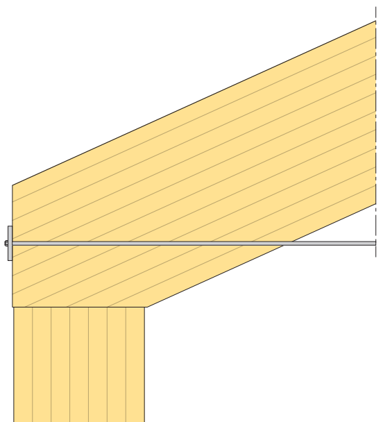
Figure 16.33 Steel tension tie fixing: Requires fireproofing
