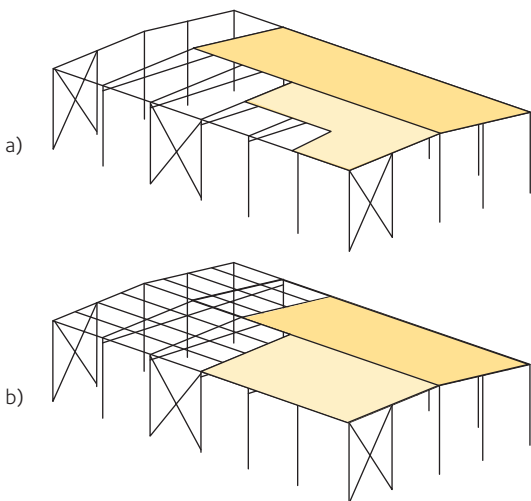
Figure 13.28 Roof diaphragm arrangements
