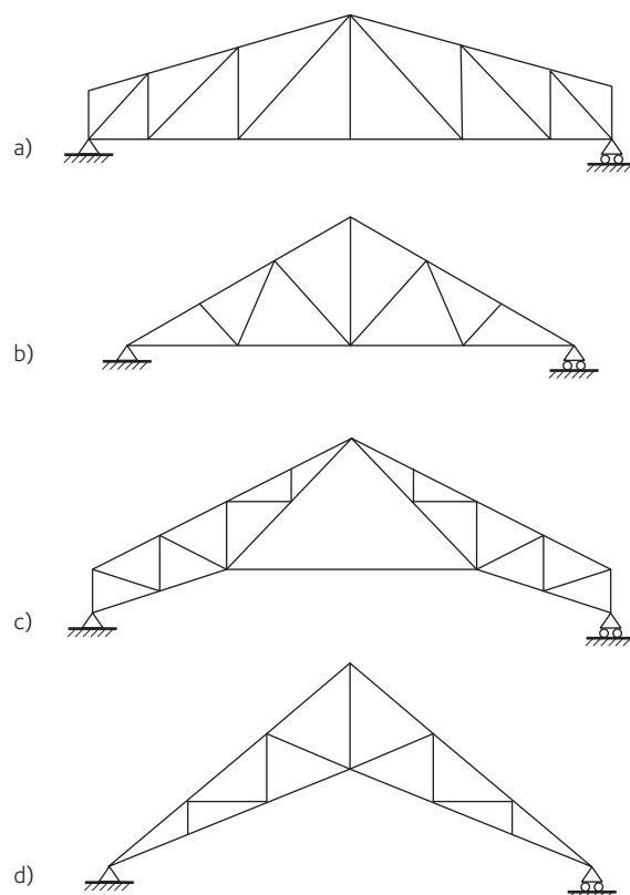
Figure 8.4 Examples of double pitched trusses
