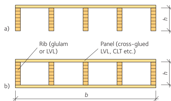
Figure 13.30 Typical cross-section of wood-based roof systems
