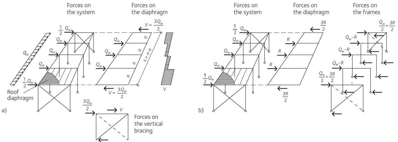
Figure 13.27 Load sharing mechanisms
