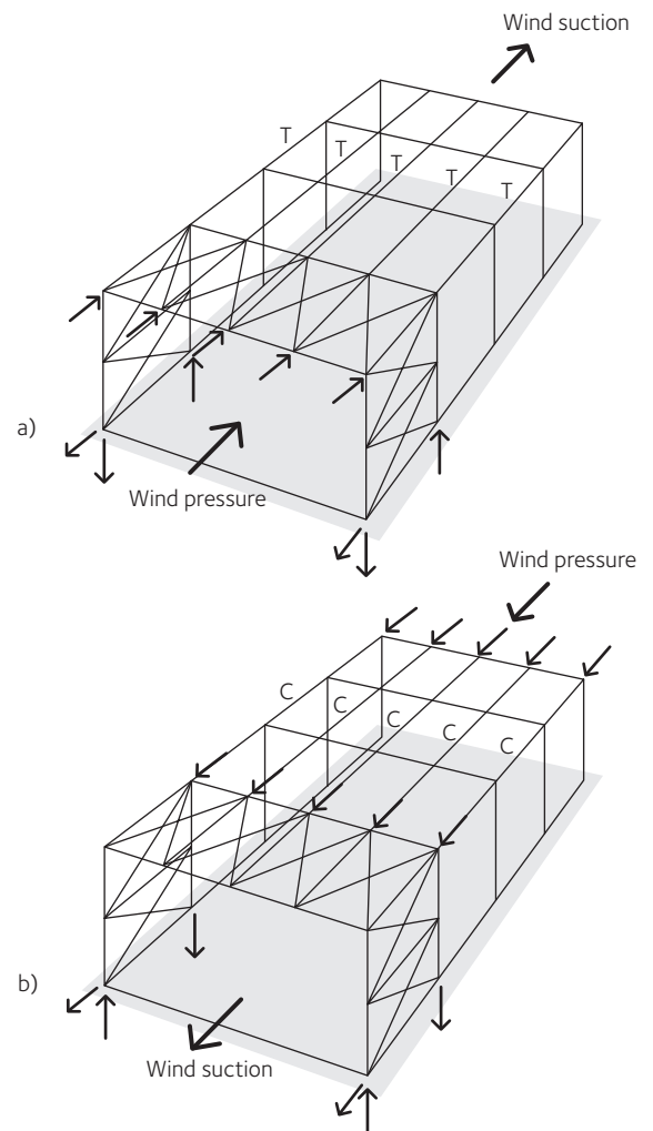
Figure 13.23 Bracing of a small building
