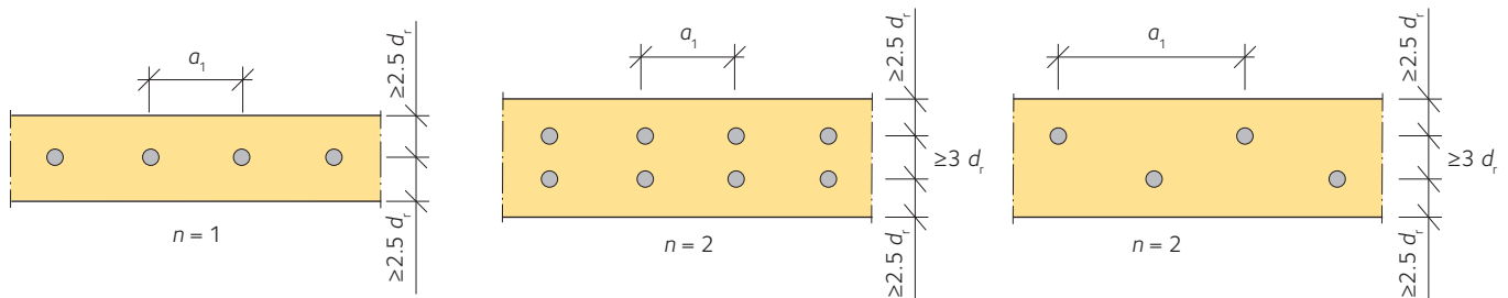
Figure 7.21 Definition of "n" and a_1 in equation 7.26 and equation 7.27 ("n" is the number of groups of reinforcement bars in the direction perpendicular to the longitudinal axis of the beam). d_r is the outer thread diameter of the reinforcement.
