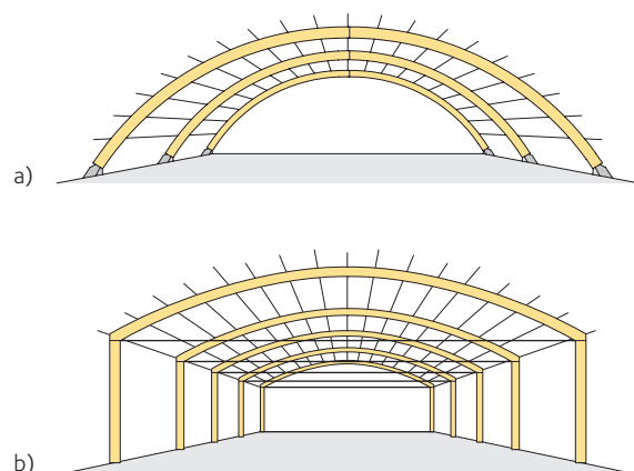
Figure 3.14 Arches
