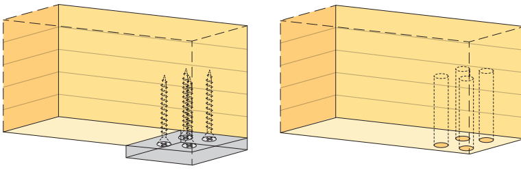
Figure 4.9 Example of a beam support reinforced for compression perpendicular to grain with self-tapping screws (left) and wooden glued-in rods (right), respectively
