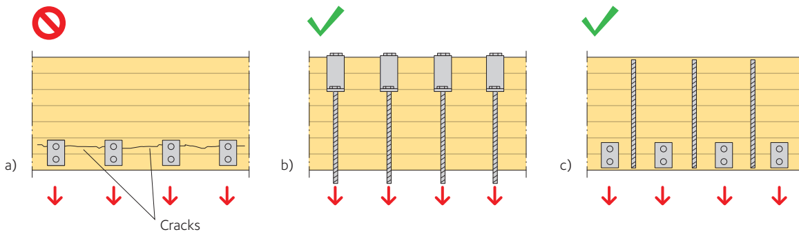
Figure 15.1 Beams subjected to heavy loads
