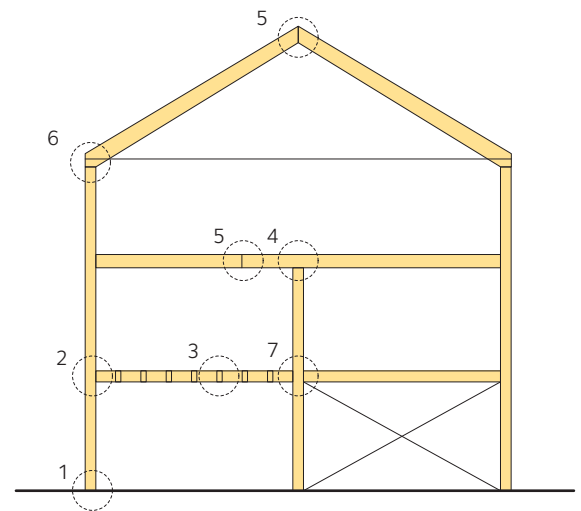
Figure 14.1 Typical connection types in a beam-column framed structure
