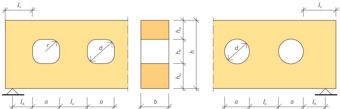
Figure 5.5 Notation for design of a beam with a rectangular or circular hole
