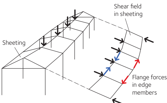
Figure 13.29 "Deep plate girder action" in pitched roof sheeting
