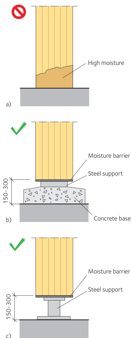
Figure 15.10 Column base
