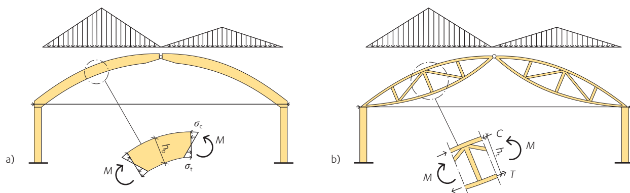
Figure 11.4 Arch structures subjected to triangular load distribution
