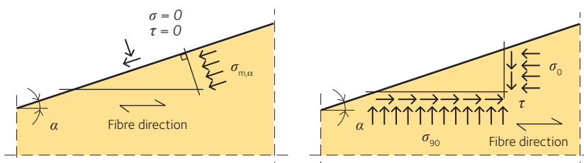
Figure 7.3 Stresses at the tapered edge of a beam
